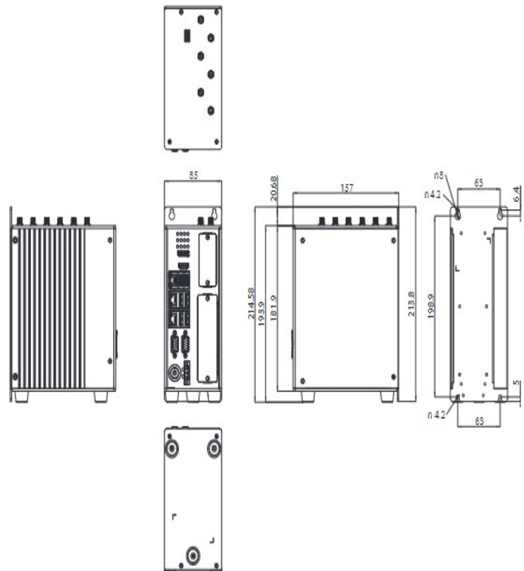
HB2-MMQB-x Mounting Diagram (Dimensions in mm)
